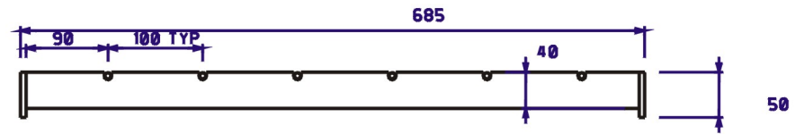
SECTION AA
